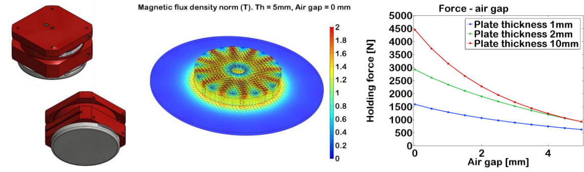
Force-air gap curve for an end effector, for various plate thicknesses
