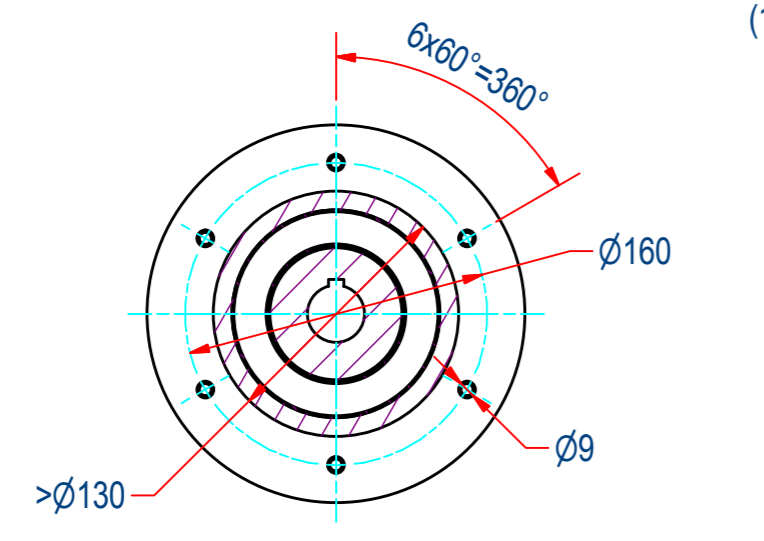
F-F MOUNTING DETAIL (2x) HOLE PATTERN COUNTER PART
