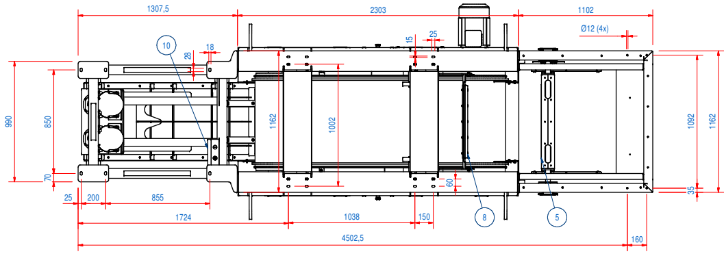
LAYOUT MOUNTING HOLES
