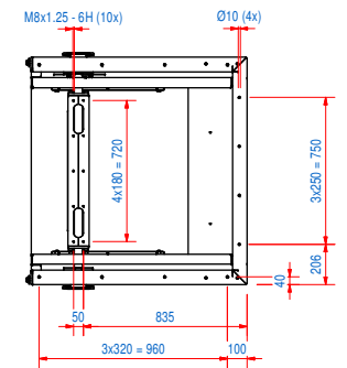
LAYOUT MOUNTING HOLES FUNNEL
