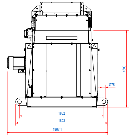
LAYOUT MOUNTING HOLES FUNNEL
