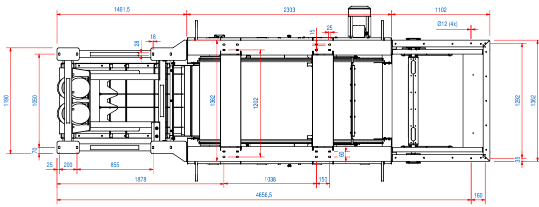
LAYOUT MOUNTING HOLES
