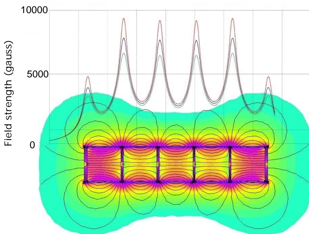
Example: Magnetic bar Ø23 mm (GSN-42) in extractor tube Ø25 mm
