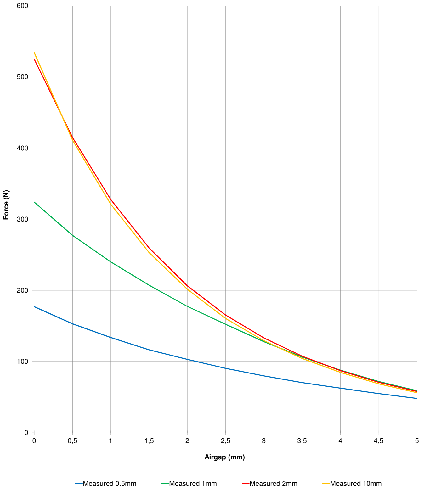
TPGC070078 Holding force curve plate thickness 0,5-10mm
