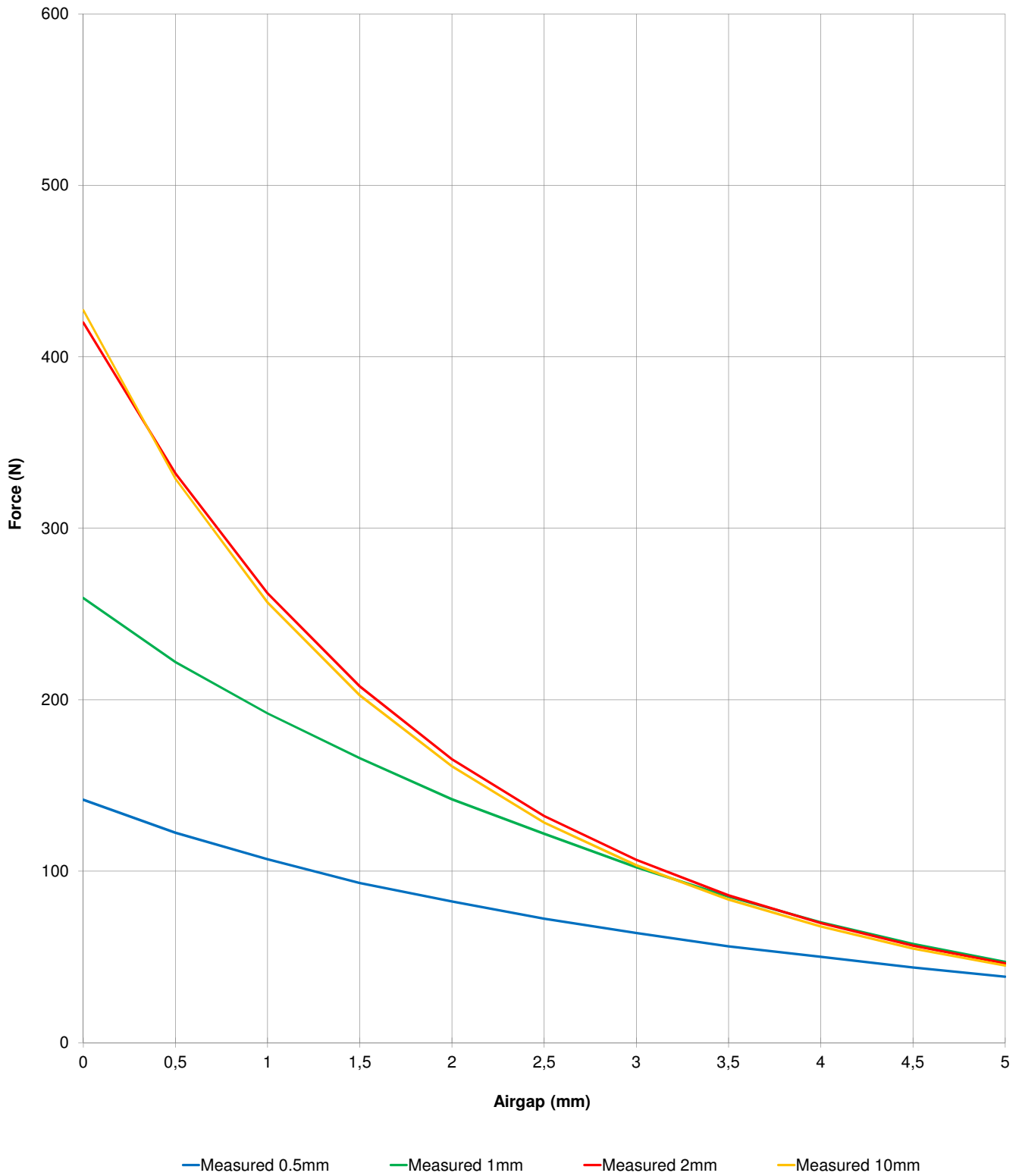
TPGC070378 Holding force curve plate thickness 0,5-10mm
