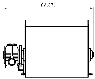
VIEW B
